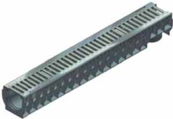
RECYFIX® 100 Surface Water Drainage Channels come with slotted, galvanised steel gratings as standard.
