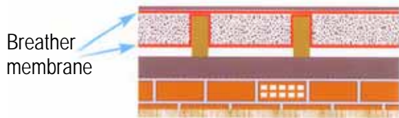
Suspended timber ground floor
